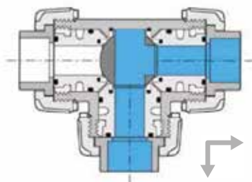
T-boring 180° open positie 2
