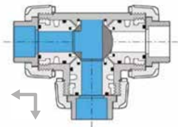
T-boring 0° open positie 1
