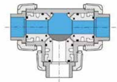
T-boring 270° open positie 4
