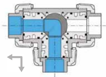
L-boring 0° open positie 1
